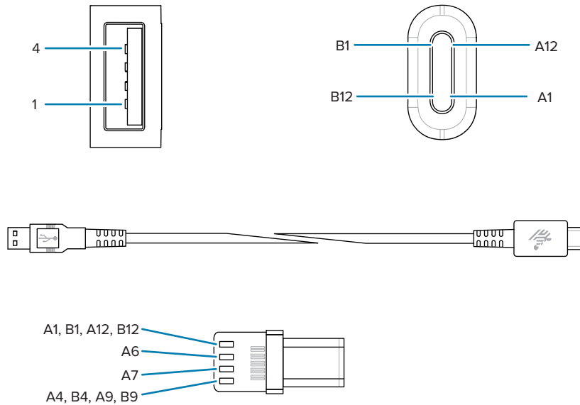
Figure 20 USB Cable
